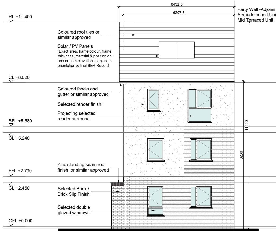
01 Front Elevation
