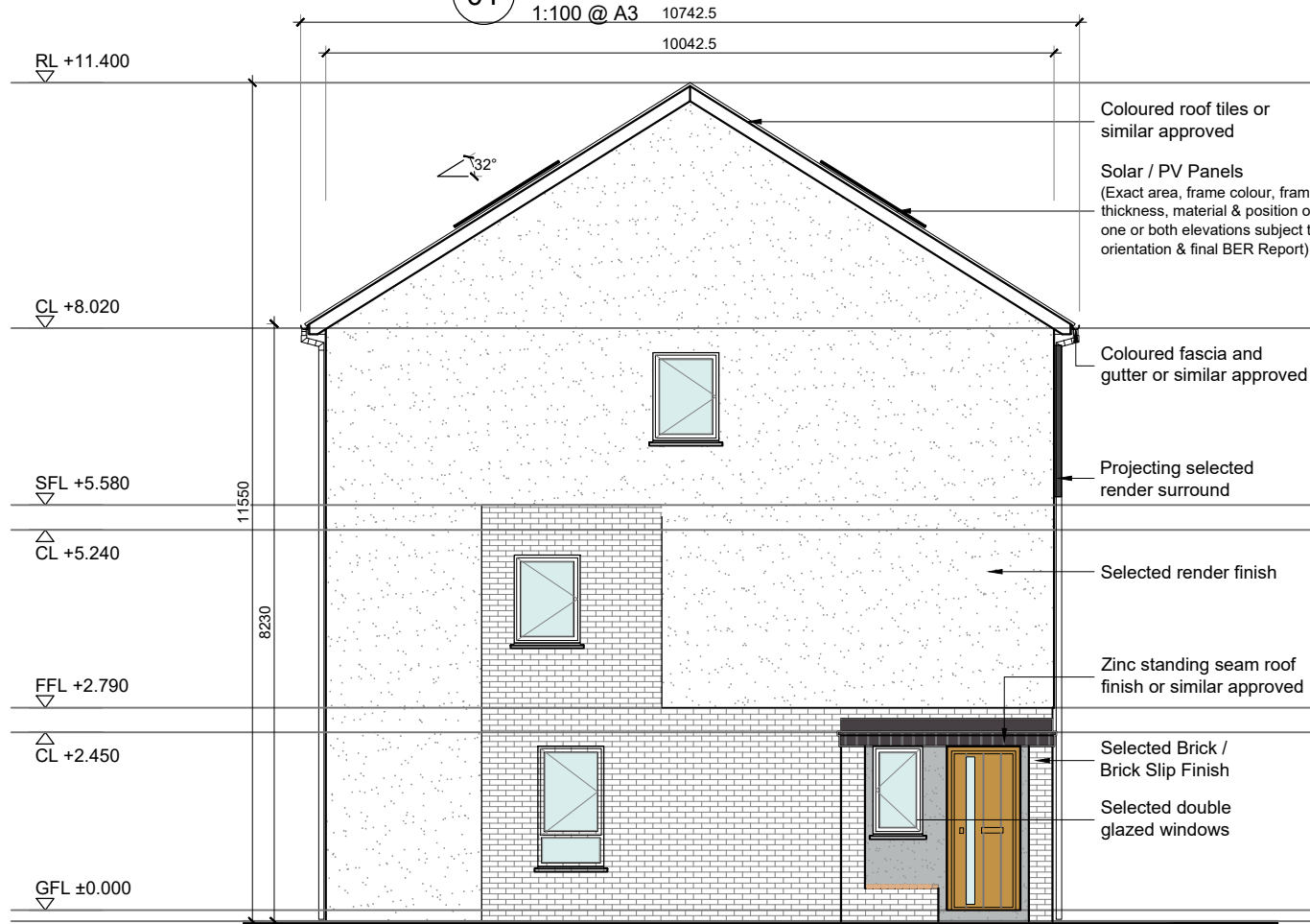
03 Side Elevation
